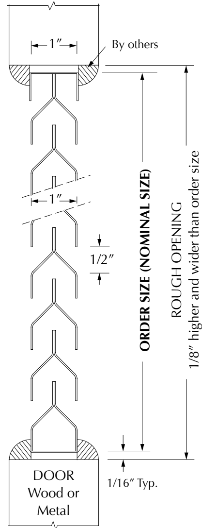
TYPICAL USER INSTALLATION. Core installed in 1 3/4” wooden door using 3/8” quarter-round.
