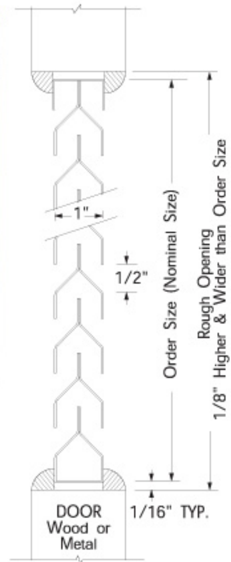
Typical user installation. Core installed in 1 3/4" wooden door using 3/8" quarter-rounds
