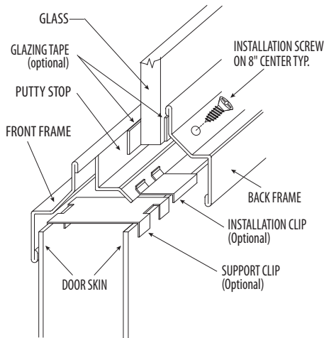
T4G Typical Construction
