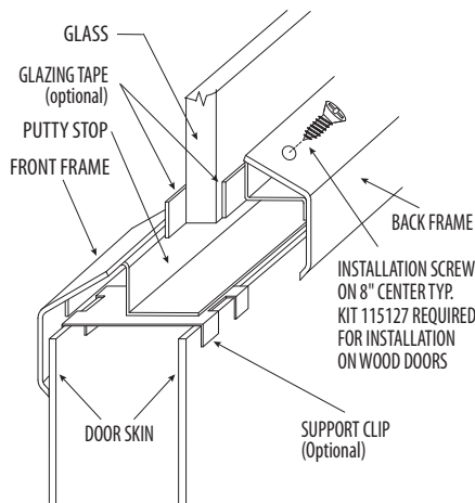
784G Typical Construction
