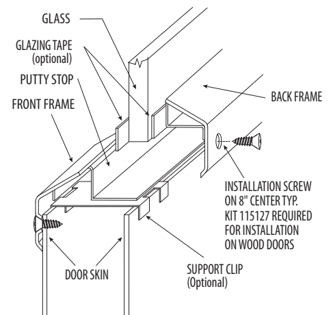
88G Typical Construction
